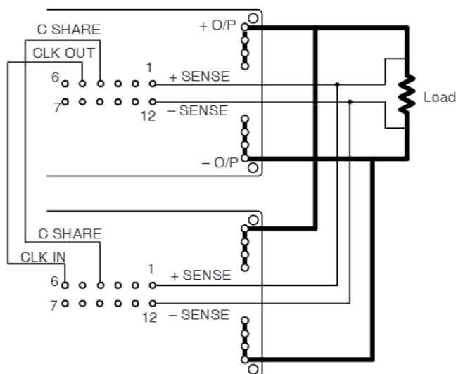
Parallel Connections
