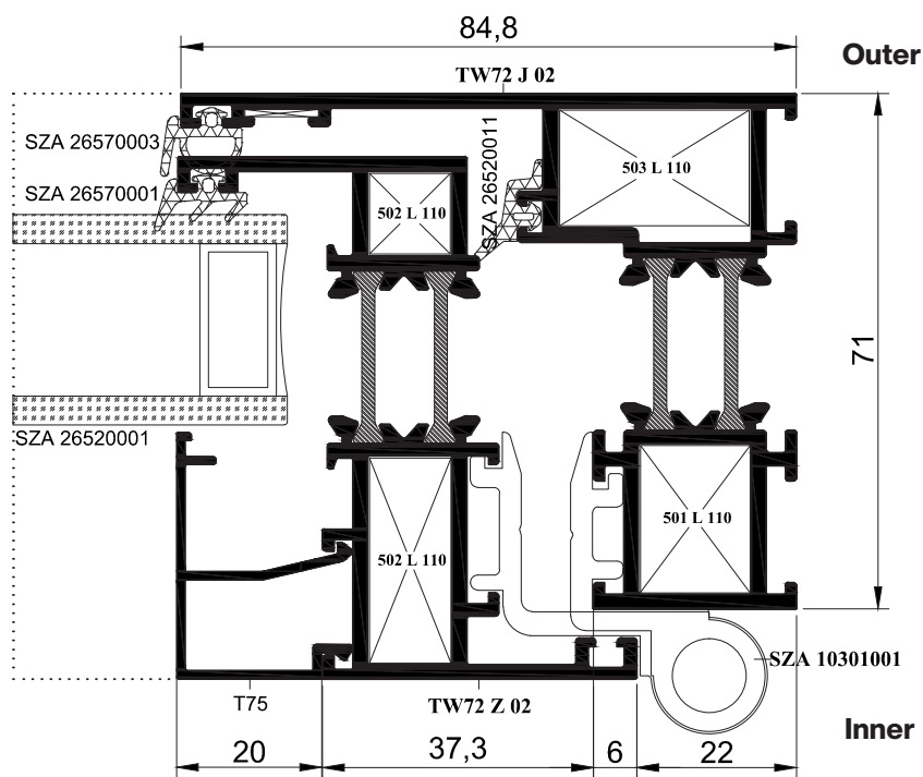
B - DETAIL
