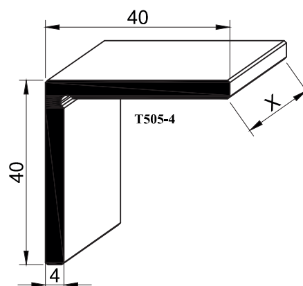
T505 - 0.818 kg/mt
