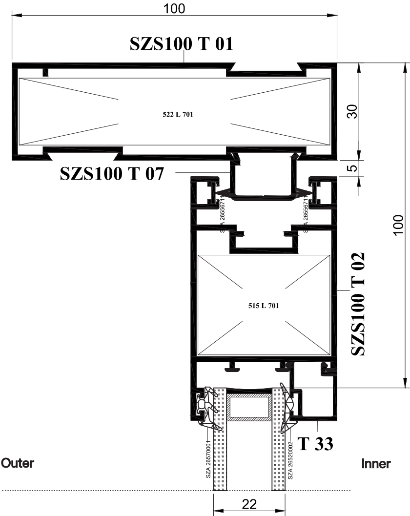
C-C DETAIL
