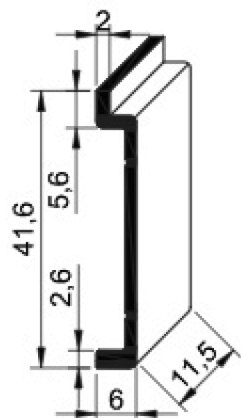
T-1076 Aluminium Joint
