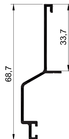
T2575 - 0.351 kg/mt
