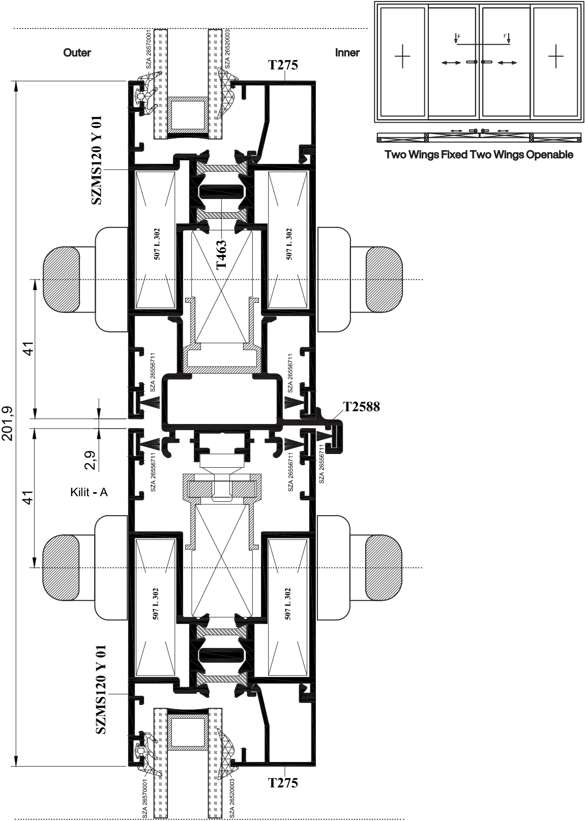
E-E DETAIL
