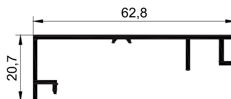
T579 - 0.388 kg/mt
