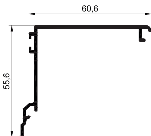
T2474 - 0.572 kg/mt
