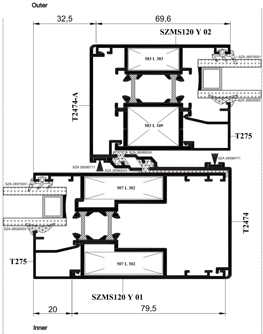
Two Wings Fixed Two Wings Openable
