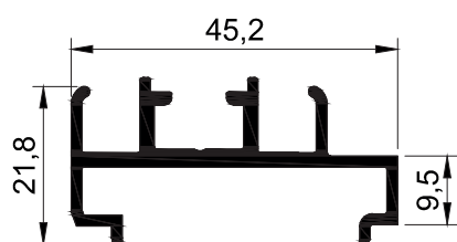
T1242 - 0.572 kg/mt
