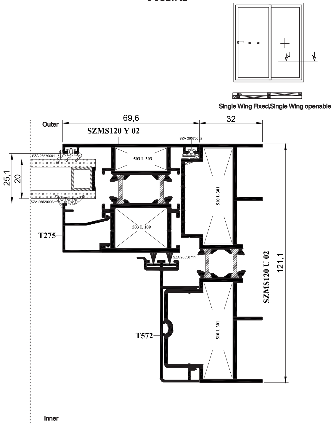
J-J DETAIL
