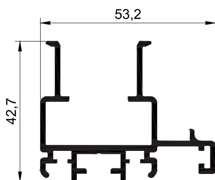
T2588 - 0.852 kg/mt
