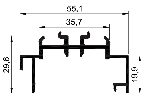
T573 - 0.667 kg/mt
