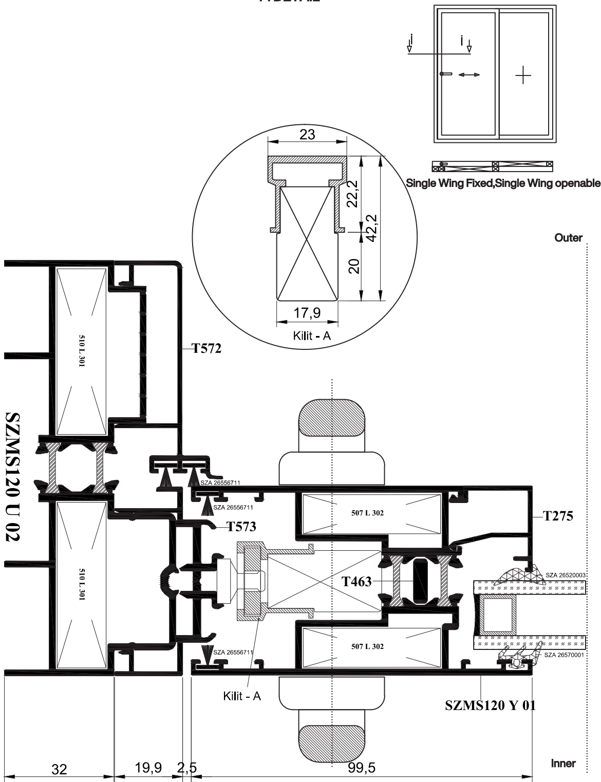
I-I DETAIL
