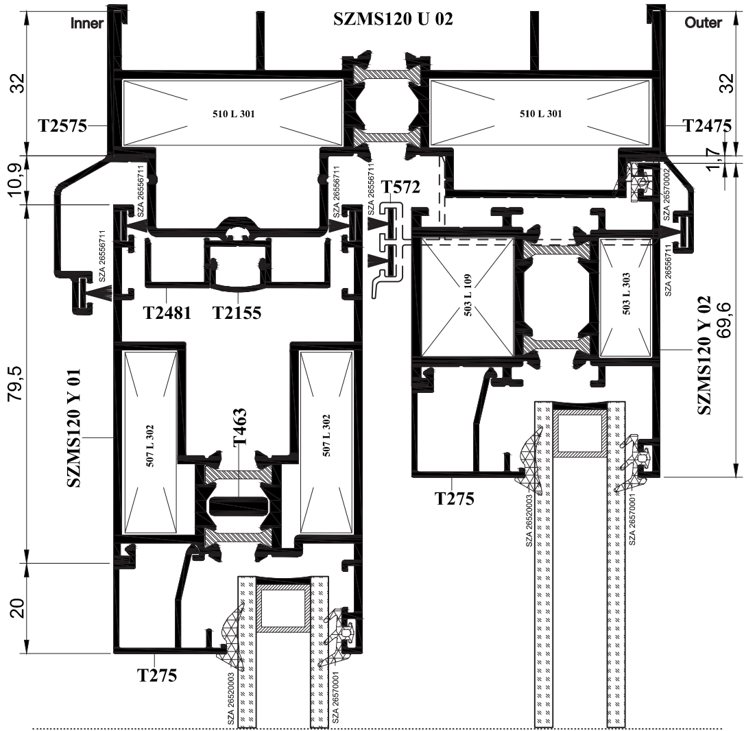
Single Wing Fixed, Single Wing openable
