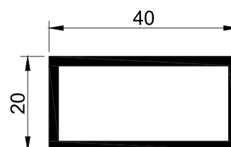
T122 - 0.609 kg/mt
