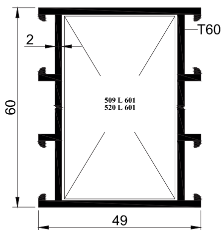
C60 T 01 -1.3mm.-0.930 kg/mt C60 T 01 -1.5mm.-0.995 kg/mt C60 T 01 -2.0mm.-1.327 kg/mt
