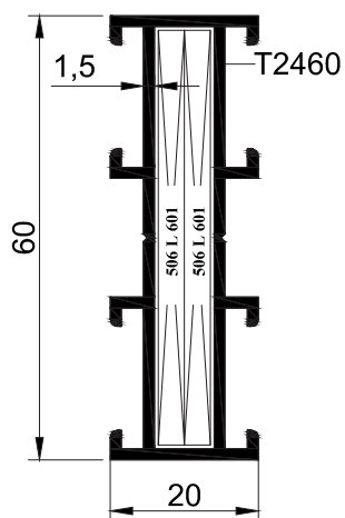
C60 T 03 -0.780 kg/mt
