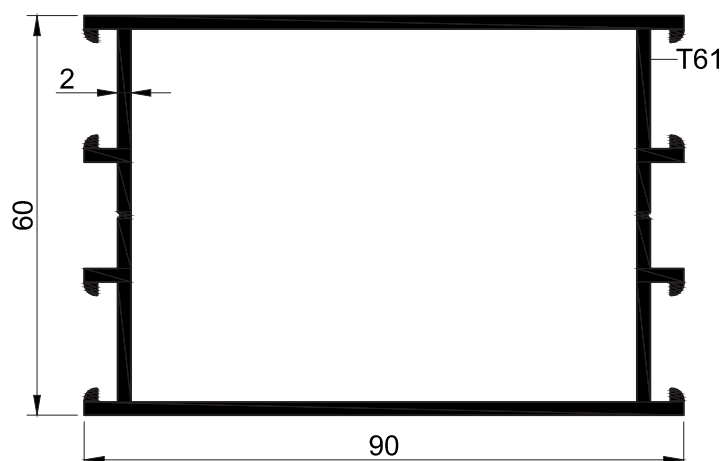
C60 T 02 -1.775 kg/mt
