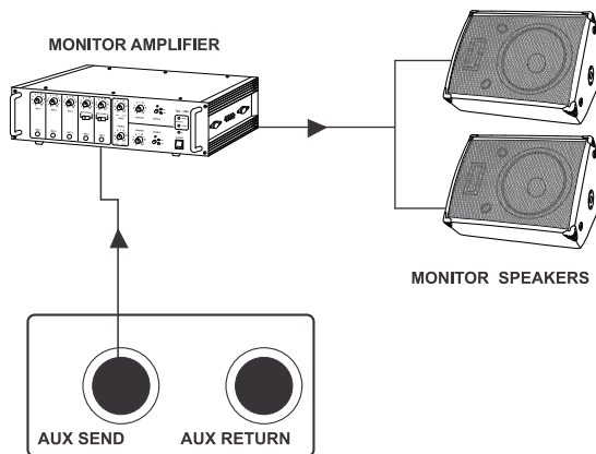
Connections for Monitor Amplifier
