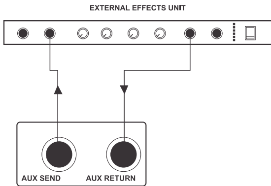
Connections for External Effects Unit
