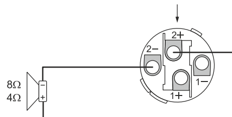
Speakon Cable Connector (Inside View)
