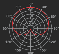
Polar Pattern
