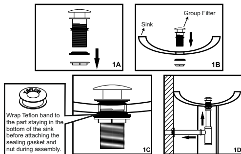
Figure 1. Flat sink flush assembly
